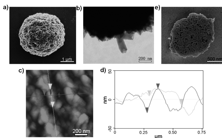
Figure 2. Morphological analysis of peptide-porphyrin microspheres. a) SEM image of a single microsphere showing irregular surface texture. b) TEM image of a microsphere showing a substructure of aggregated nanorods and nanotubes. c) AFM contact-mode height image with line profiles (light gray and gray lines) showing the presence of closely packed nanorods; and d) corresponding height profiles confirming the presence of elongated nanostructures on the microsphere surface (x axis: distance, y axis: height). e) SEM image of a single microsphere cross-section showing porous, multi-chambered interior.
